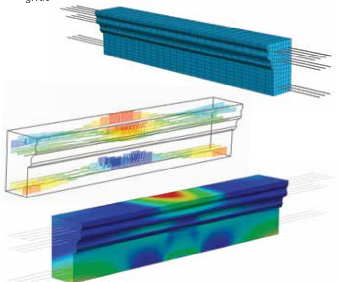
3D dynamic analysis of a reinforced lintel showing stress and strain
