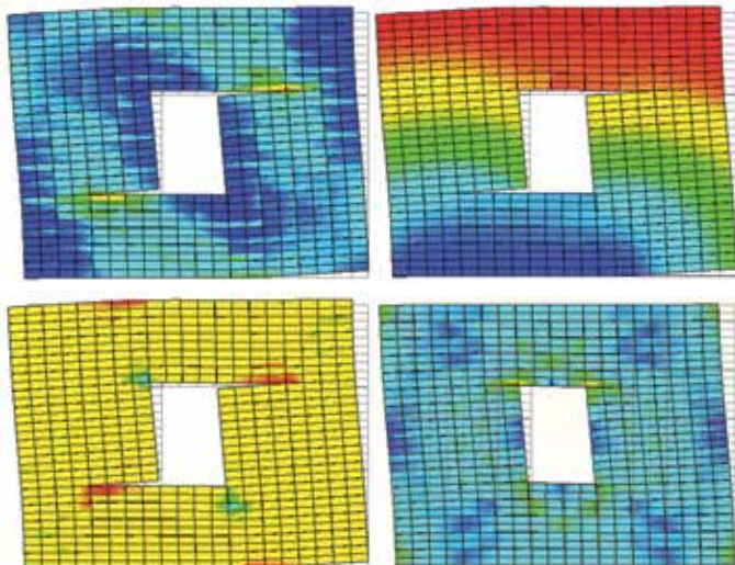
Discrete masonry modelling
