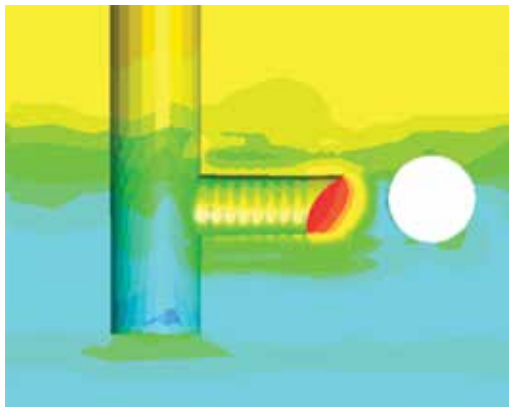
3D view of a partially excavated cross-passage and tunnel tube*
