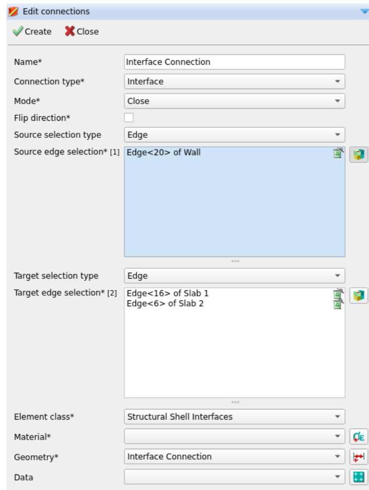
Figure 4: Connection assignment
