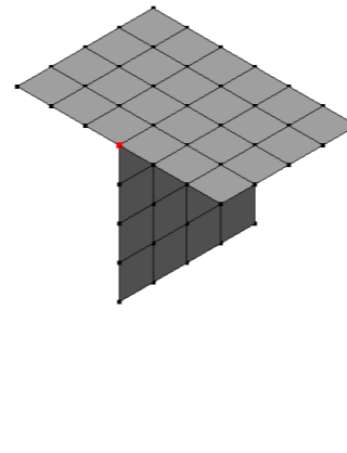
Figure 12: Point selected for checking node count
