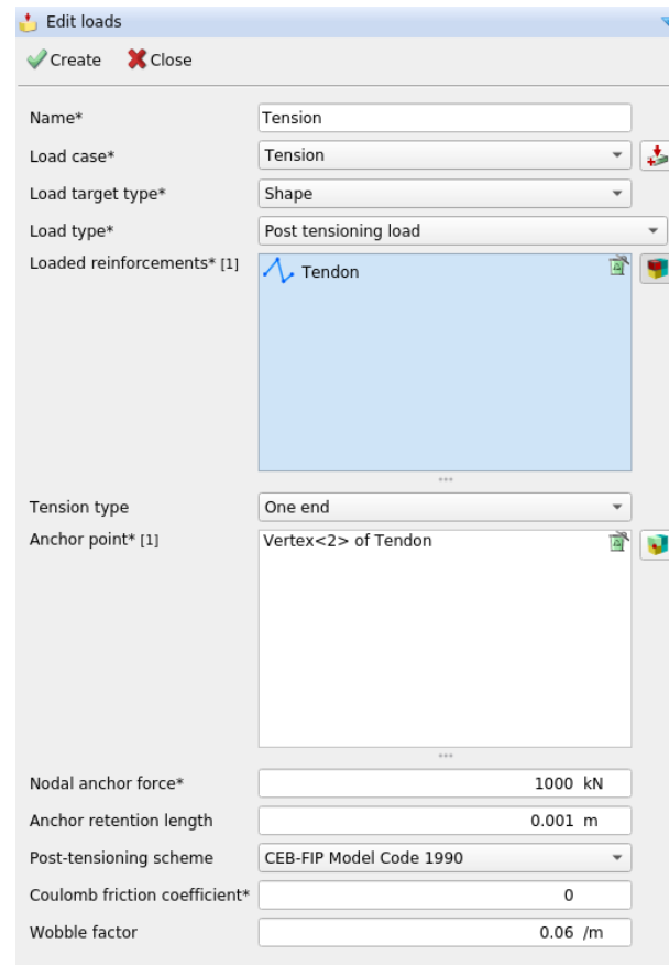
Figure 14: Post-tensioning load with anchorage loss input
