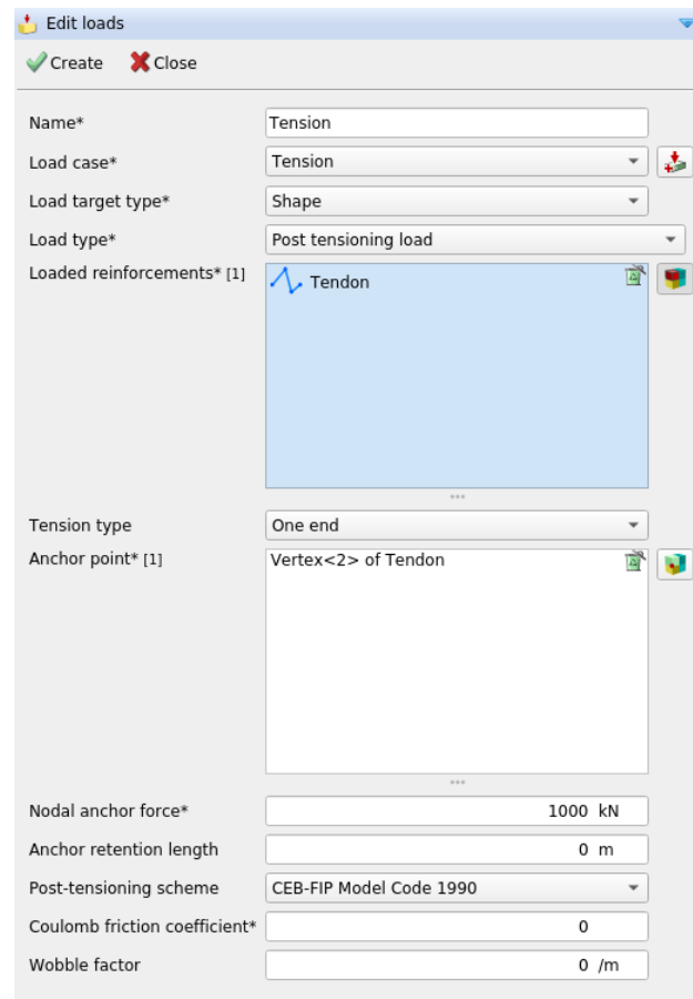
Figure 2: Define post-tensioning load
