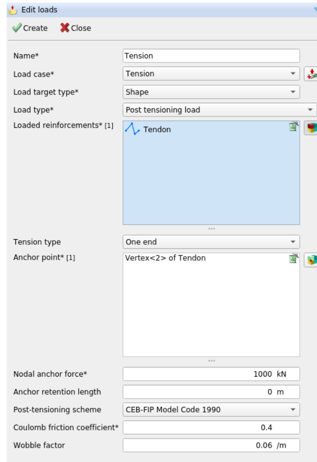
Figure 11: Post-tensioning load with friction loss
